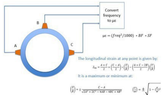
System Setup
